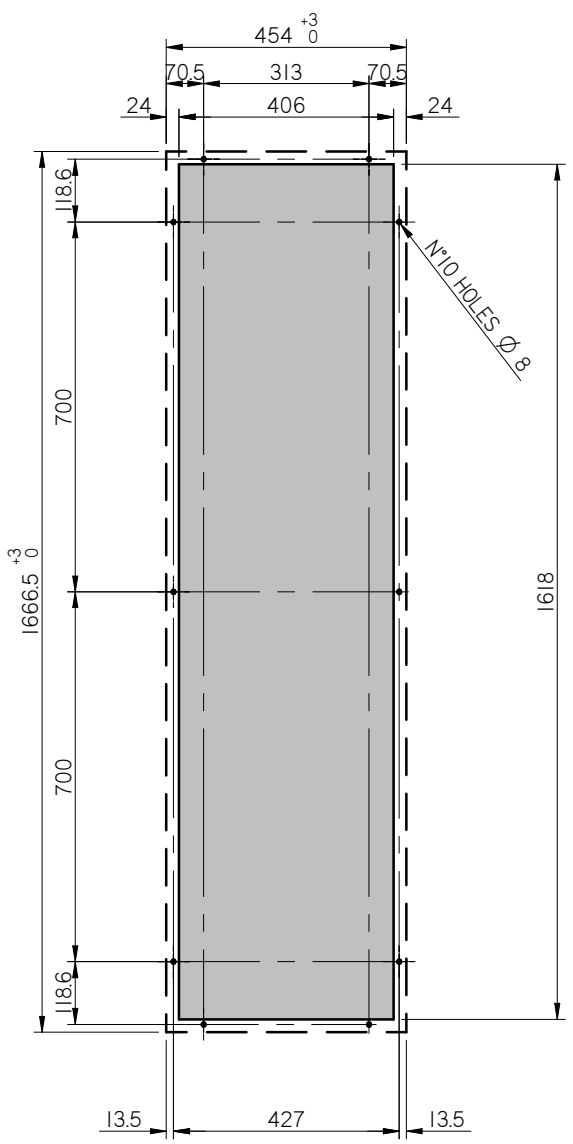
MONTAGGIO A INCASSO / SEMINCASSO FLUSH / SEMI-FLUSH MOUNTING
